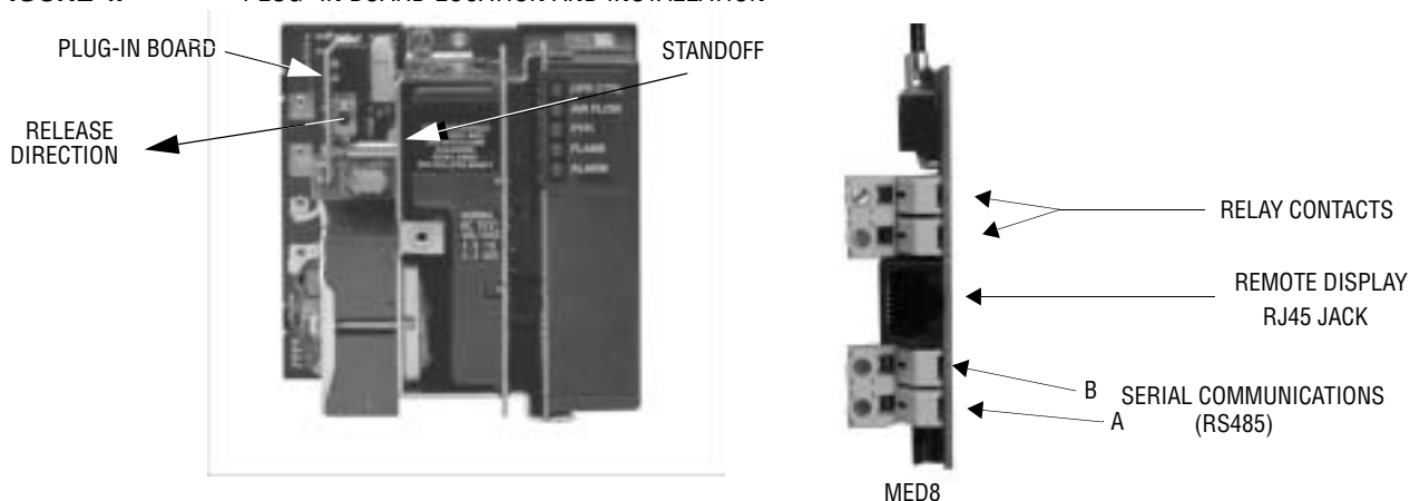
FIGURE 4. PLUG -IN BOARD LOCATION AND INSTALLATION
