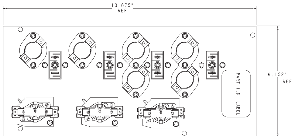
Mounting plate width is 13.875" on current ECB29-12.5 and 15kw electric heat sections
