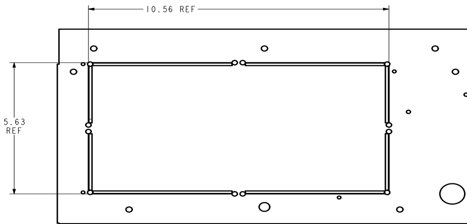
CB29M-31 electric heat section opening width is 10.56"
