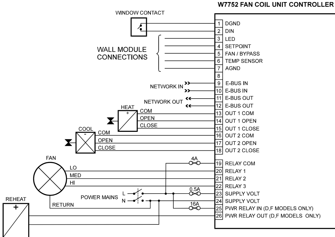
Fig. 4. Input/output details.
