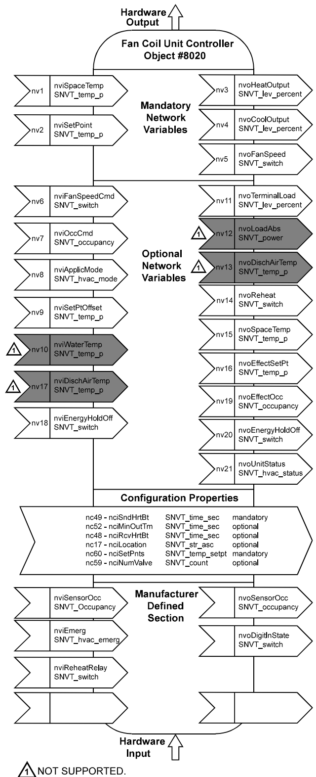
Fig. 3. LonMark object details.
